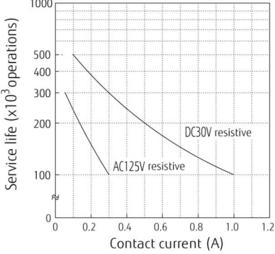
Life curve
